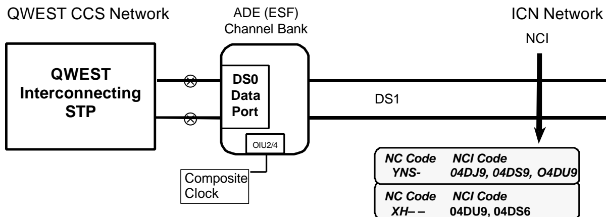
Figure 4-1 Qwest STP Equipped with a DS0-A Port
