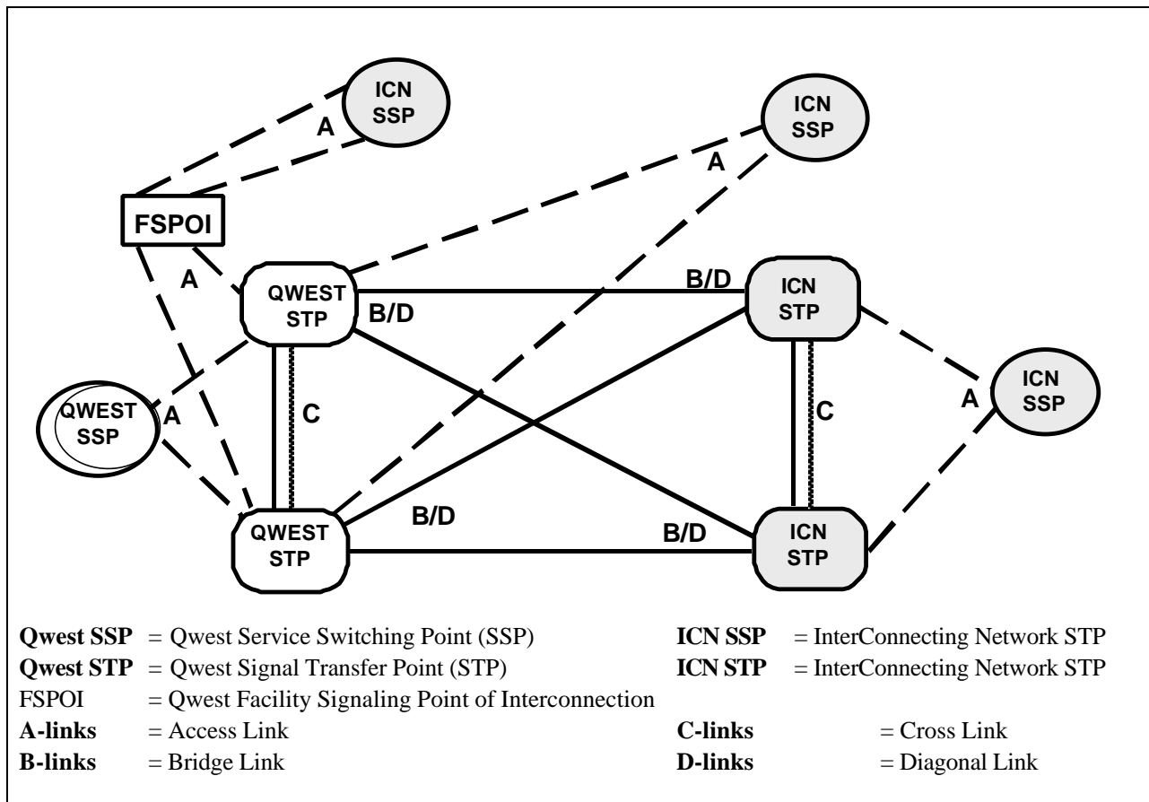
Figure 2-1 CCS Network Interconnection Architecture
