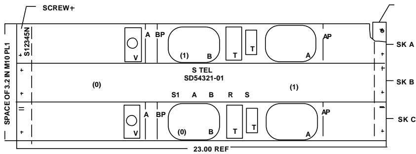
Figure 3-P Equipment Assembly, Mounting Plate Unit-Main View (With Stocklist)
