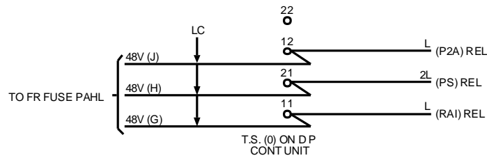
Figure 2-19 Cabling Diagram
