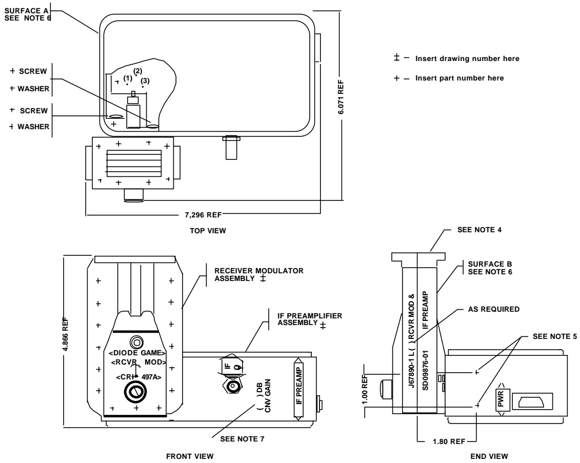
Figure 3-N Equipment Assembly, Chassis Unit-Main View (With Stocklist)
