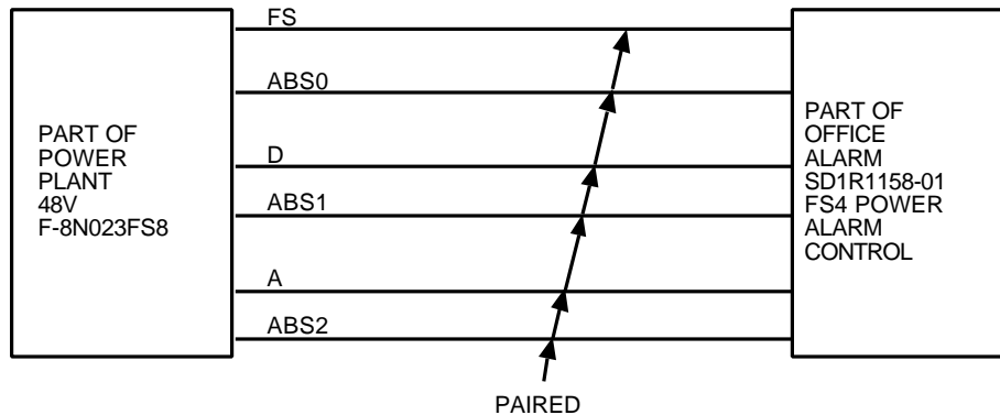
Figure 2-20 Block Diagram
