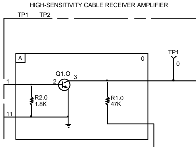
Figure 2-21 Sample Circuit Pack Schematic
