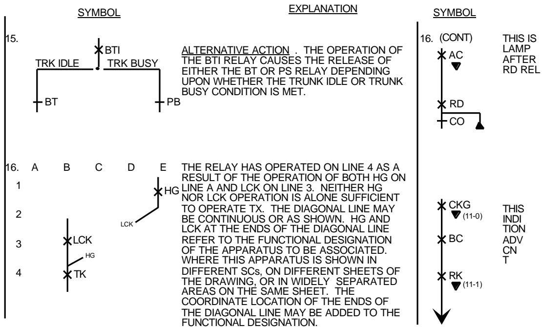
Figure 2-15 Sequence Chart
