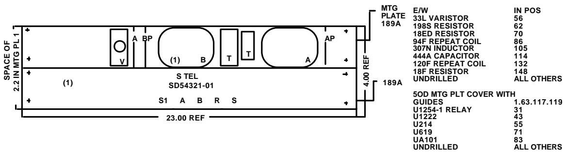
Figure 3-R Equipment Assembly, Mounting Plate Unit - Main View (Without Stocklist)
