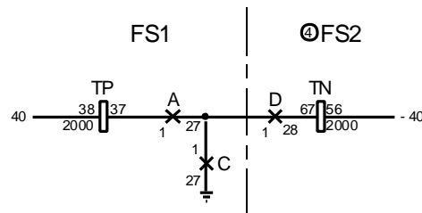
Figure 2-8 Functional Schematic
