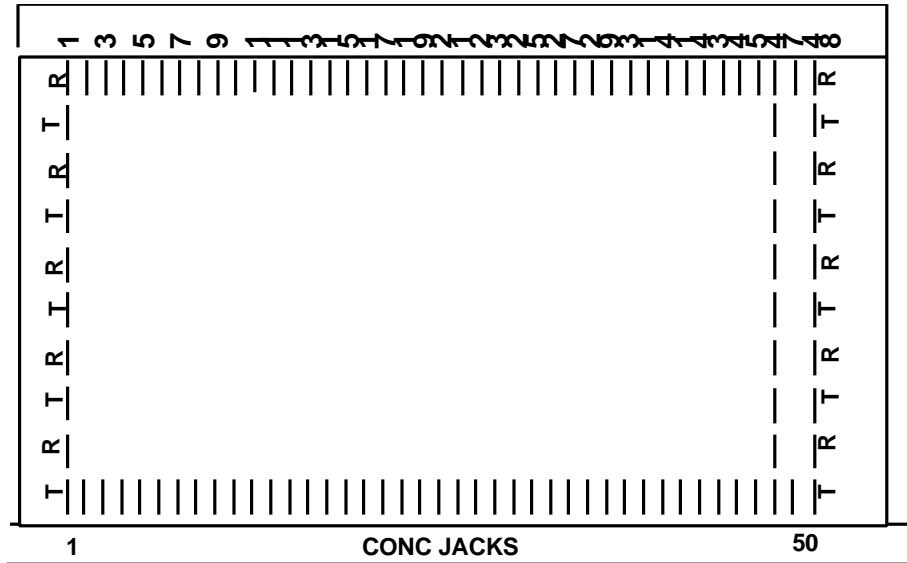
Figure 3-CC Method of Showing Terminal Strips and Terminals
