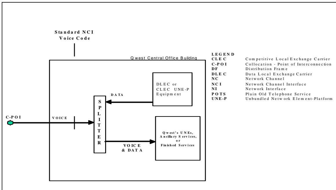
Figure 2-6 DS0 FC Collocation, Example 3
