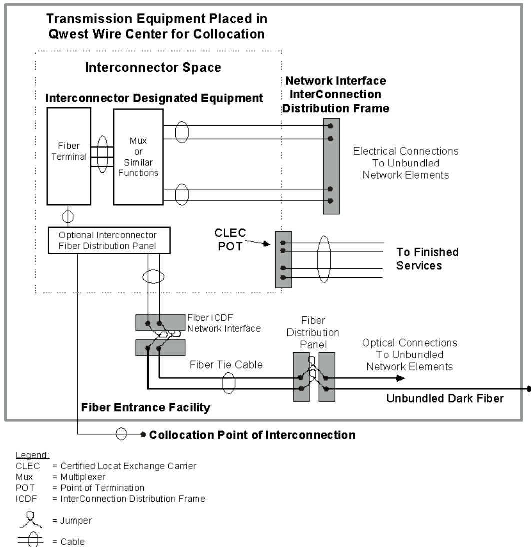
Figure 12-1: Fiber ICDF Arrangement
