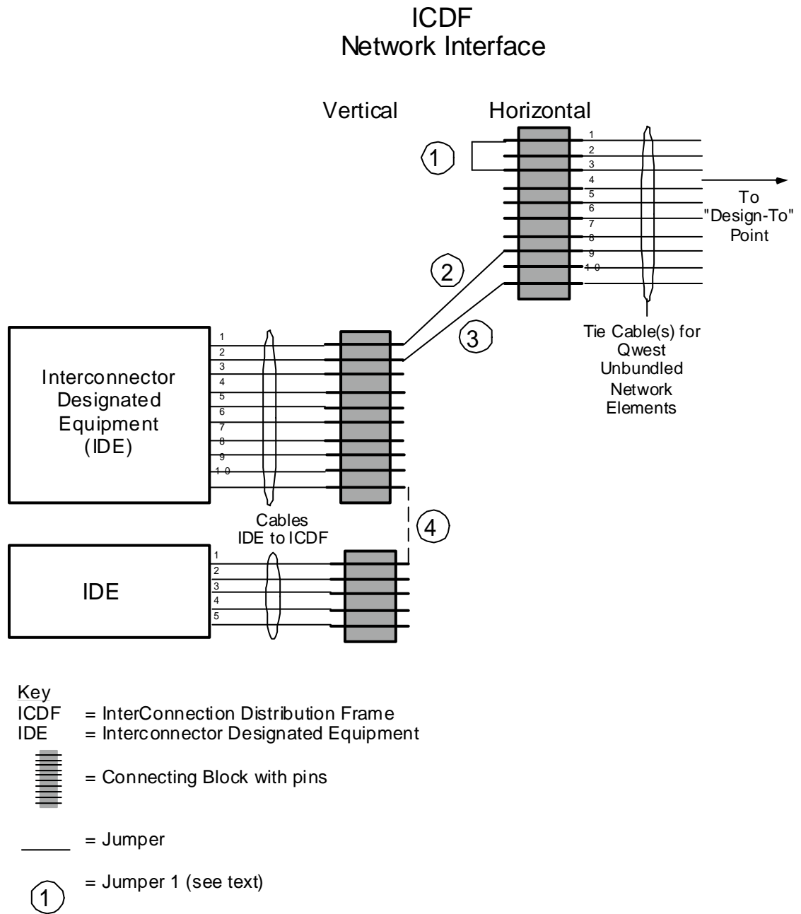
Figure 3-3 Generic DS0/Voice Interconnection Arrangement
