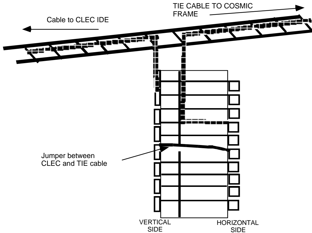
End view of InterConnection Distribution Frame (ICDF) showing typical CLEC cable termination, a jumper between the horizontal and vertical side, and a typical tie cable termination.
