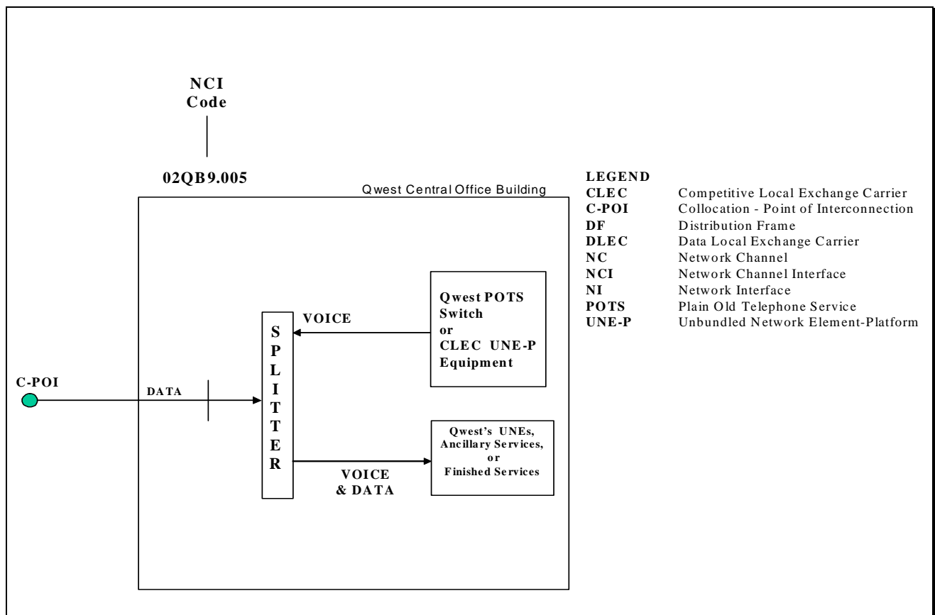
Figure 2-4 DS0 FC Collocation, Example 1
