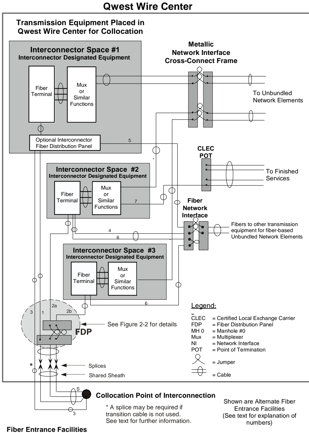
Figure 2-1 Fiber Entrance Facility Arrangements
