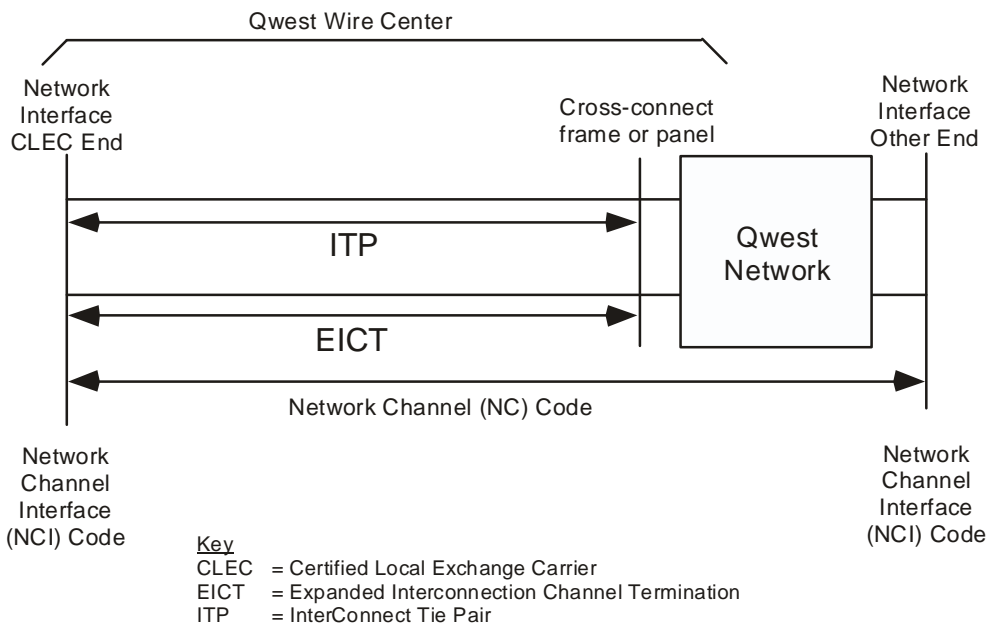
Example of Private Line Transport Service Illustrating an Expanded Interconnection Channel Termination (EICT)
