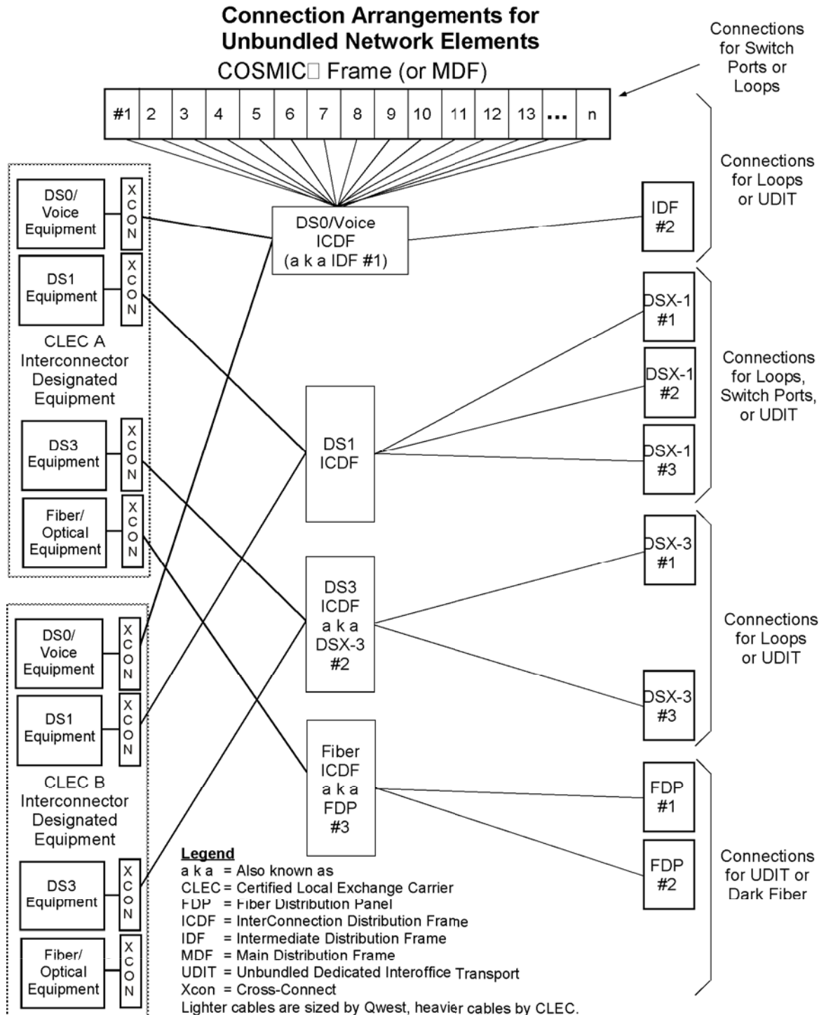
Figure 3-8 Typical Standard ICDF Arrangement
