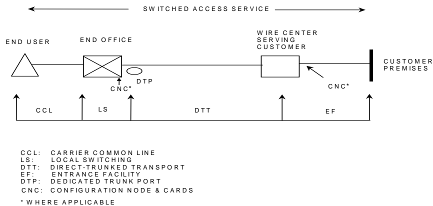
(B) OptiPoint Service without Telephone Company Provided Terminal Equipment at the Customer Premises
