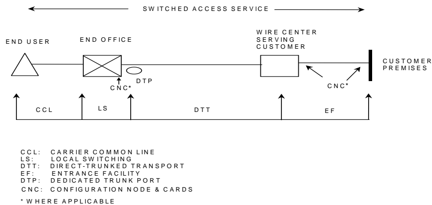
(A) OptiPoint Service with Telephone Company Provided Terminal Equipment at the Customer Premises
